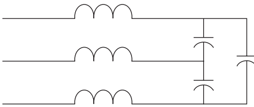
FIGURE 30.9 Typical passive filter design.
