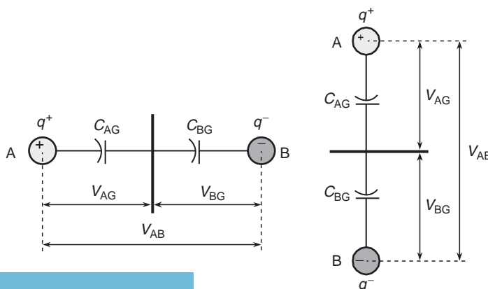
FIGURE 13.16 Capacitance between line to ground in a two-wire single-phase line.
