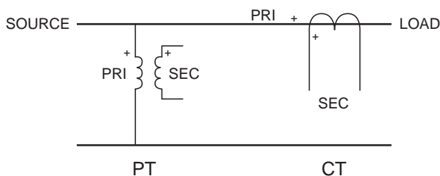
FIGURE 25.5 Instrument transformer symbols.
