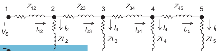
FIGURE 21.29 Linear ladder network.
