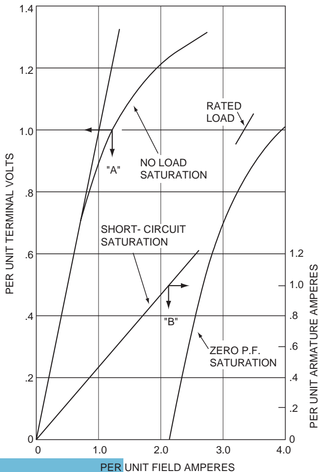
FIGURE 5.2 Saturation curves.
