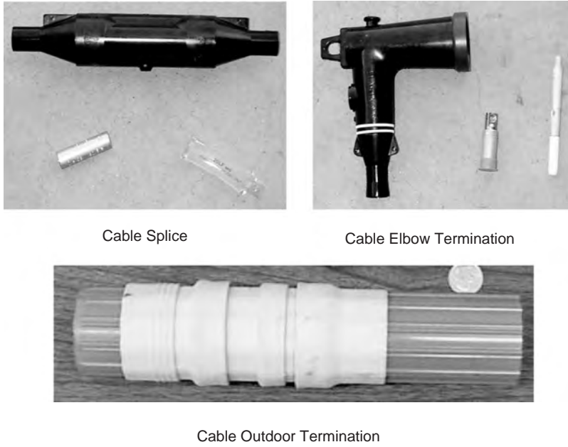
FIGURE 12.5 Cable accessories.
